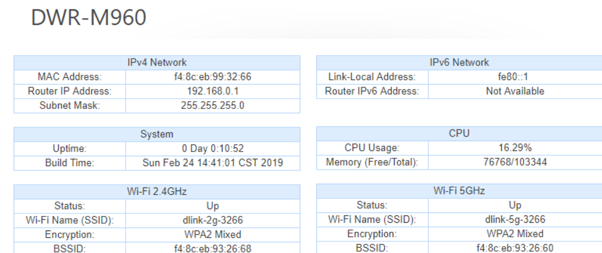
Figure 5-1-3 DWR-M960 Info
