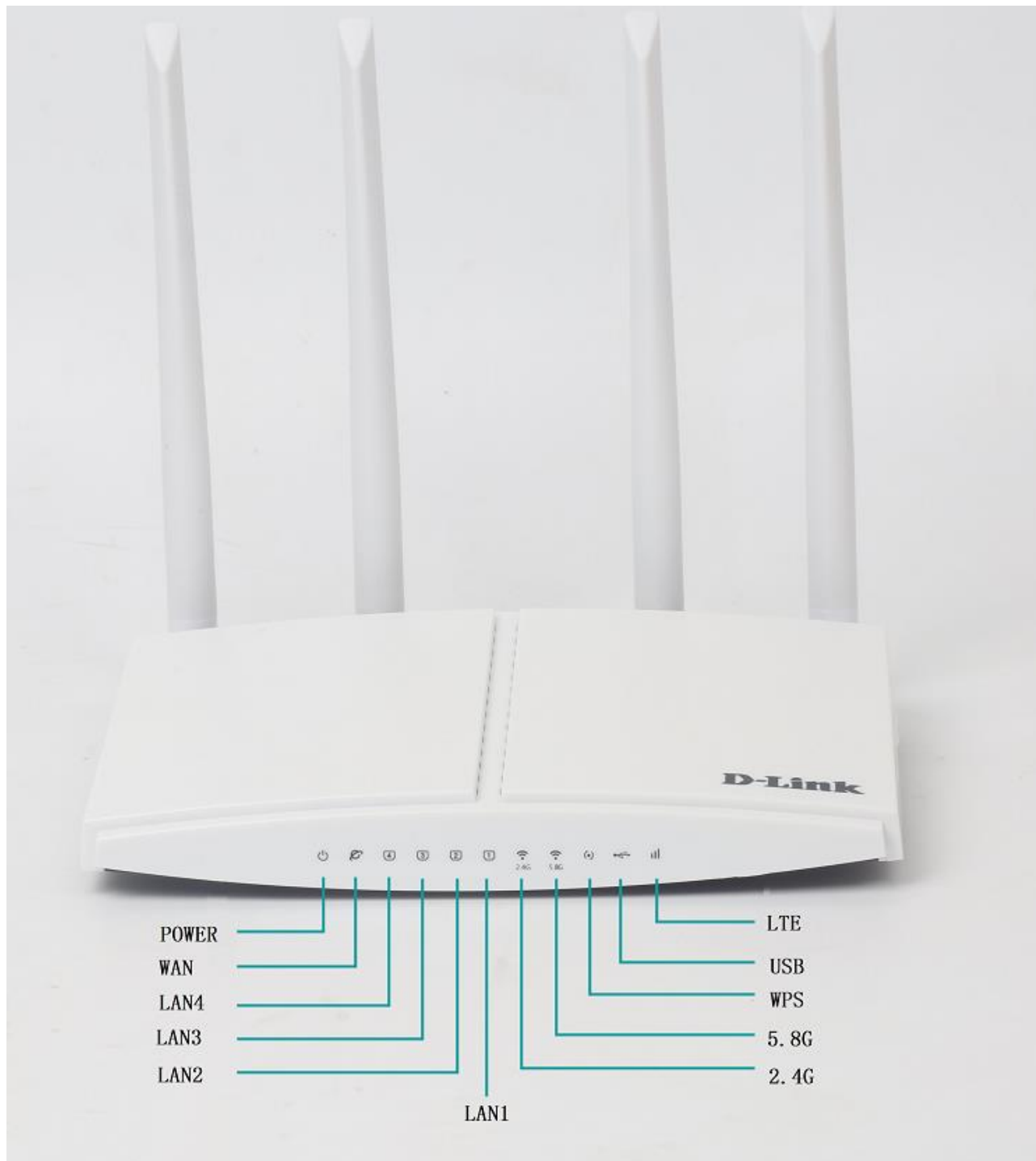
Figure 2-1-1 DWR-M960 Top View
