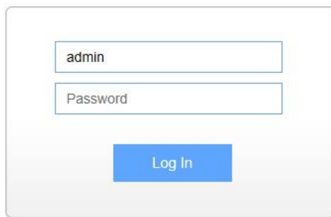
Figure 4-10 Login Window
