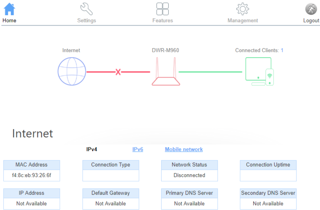
Figure 5-1 Router’s Functions
