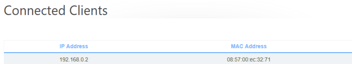
Figure 5-1-5 Connected Clients
