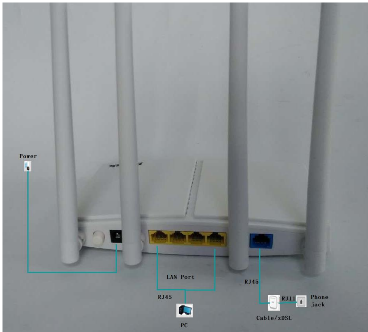
Figure 3-1 Hardware Installation of the DWR-M960 Wireless Router
