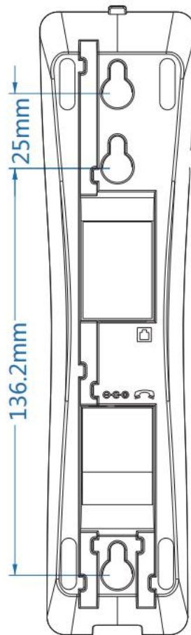
Picture 1 - Device installation
