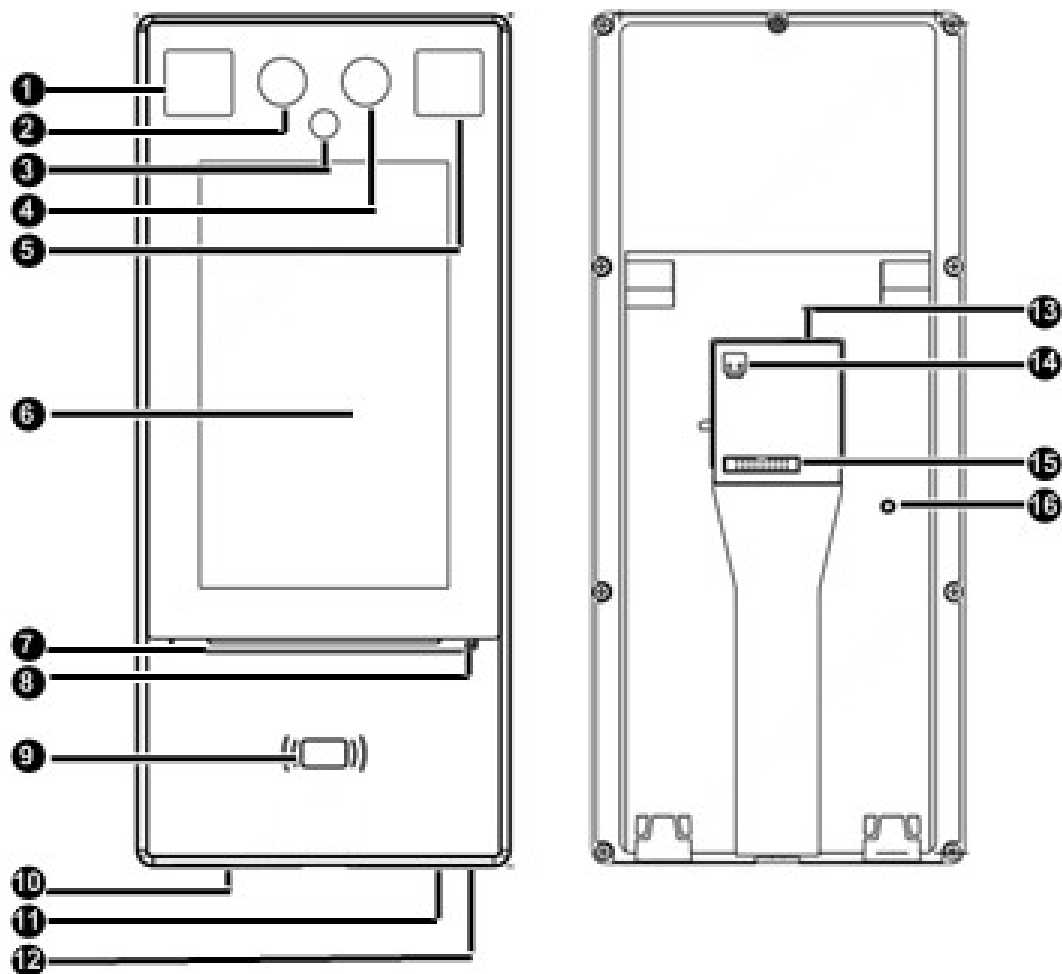
Figure3-4 Device Structure
